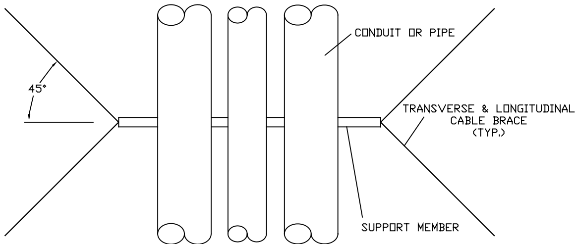
PLAN VIEW OF BRACE
