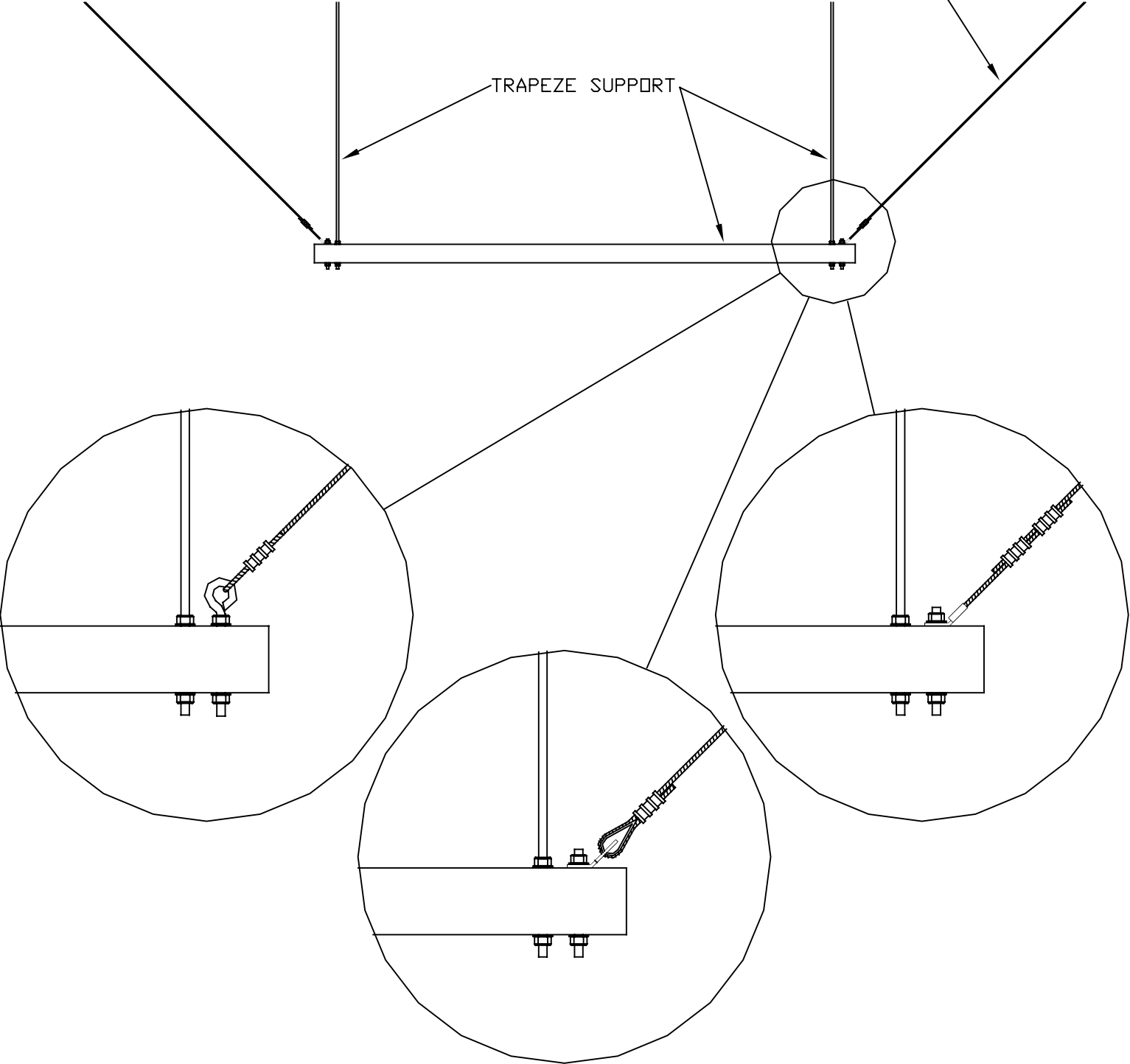
TRANSVERSE AND 4-WAY SEISMIC BRACING OF TRAPEZE SUPPORTS
