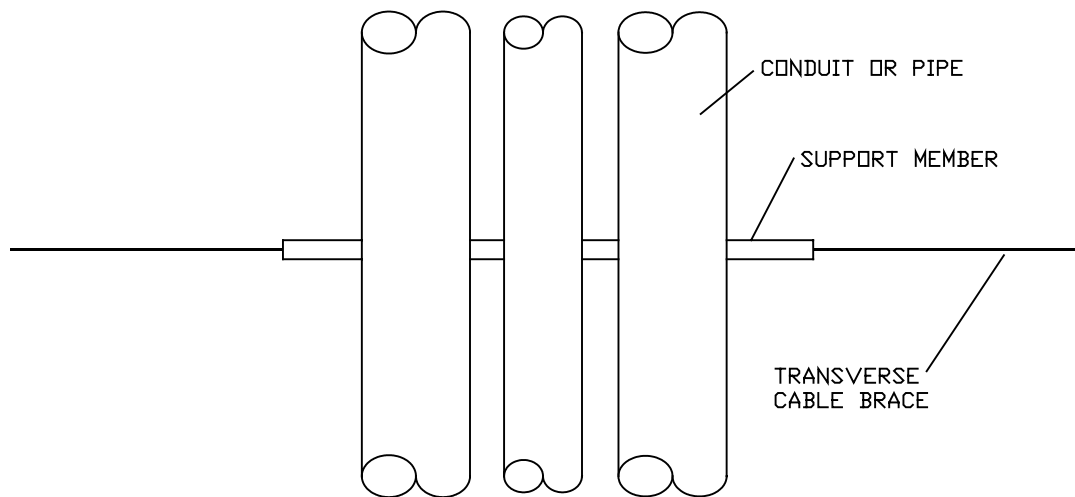
PLAN VIEW OF BRACE
