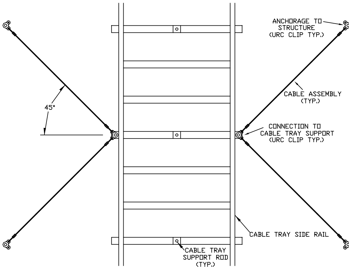
PLAN VIEW
